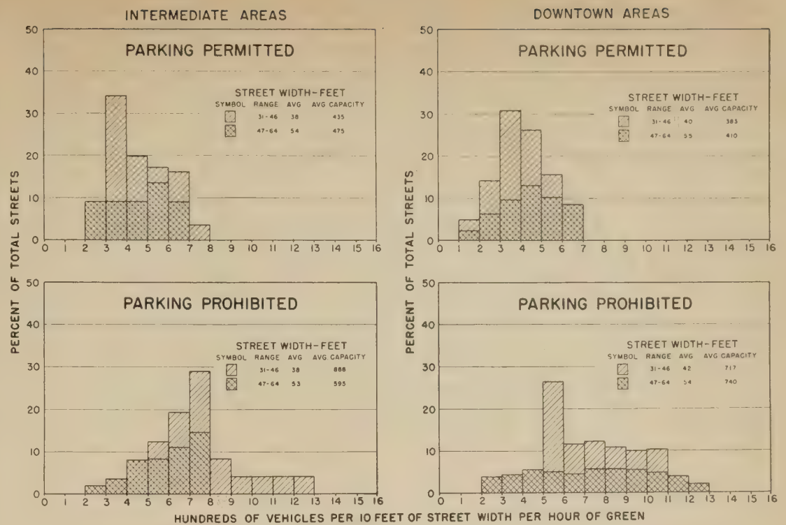
Figure 23.—Frequency distribution of intersection capacities.
